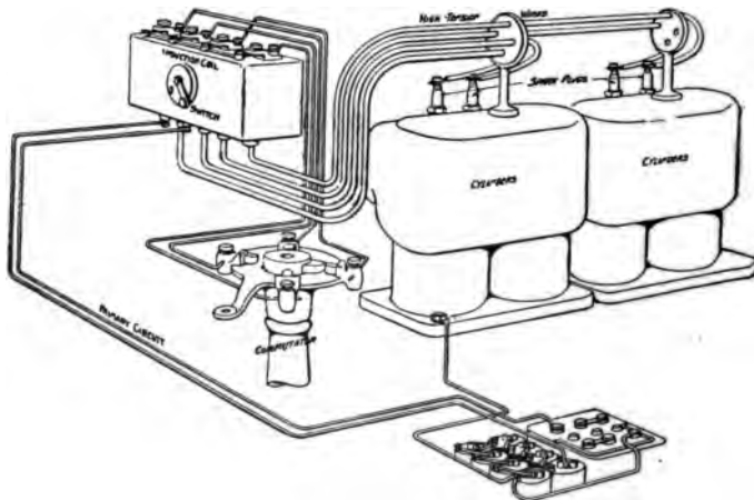
FIG. 220.—Wiring Lay-out for a Four-cylinder Engine, showing dry cell and secondary batteries, controlled by switch on coil-box.
